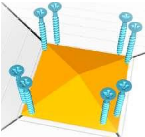
11. roof top with 4.0x40 screws
