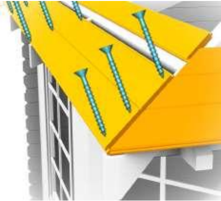
11. roof top with 4.0x40 screws
